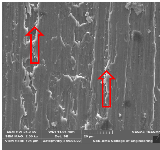
Figure 11 worn-out surfaces for the Inconel 625- Cr 3 C 2 -NiCr coatings for the speed of 400 rpm and load of 20N
