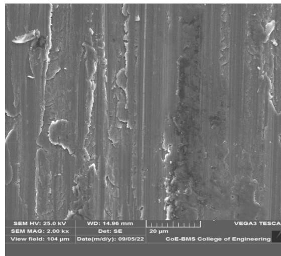
Figure 14 worn-out surfaces for the Inconel 718- \text{Cr}_3\text{C}_2 -NiCr coatings for the speed of 400 rpm and load of 20N
