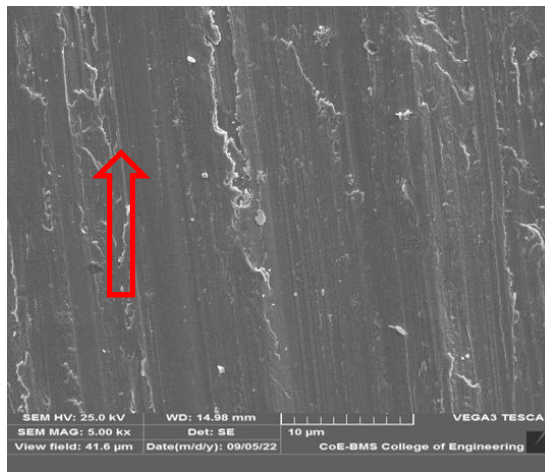
Figure 6 worn out surfaces for the Inconel 600- Cr_3C_2 -NiCr coatings for the speed of 200 rpm and load of 20N
