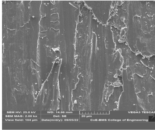
Figure 8 worn-out surfaces for the Inconel 600- Cr 3 C 2 -NiCr coatings for the speed of 400 rpm and load of 20N
