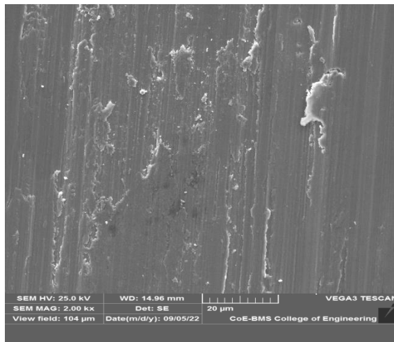
Figure 9 worn-out surfaces for the Inconel 625- Cr 3 C 2 -NiCr coatings for the speed of 200 rpm and load of 20N
