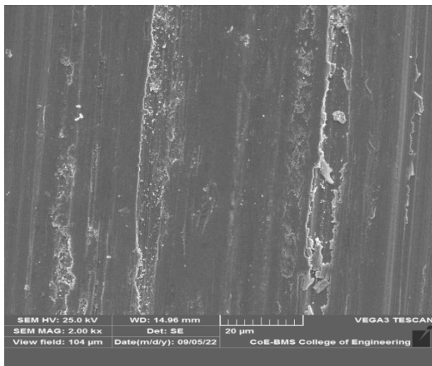
Figure 12 worn-out surfaces for the Inconel 718- Cr 3 C 2 -NiCr coatings for the speed of 200 rpm and load of 20N
