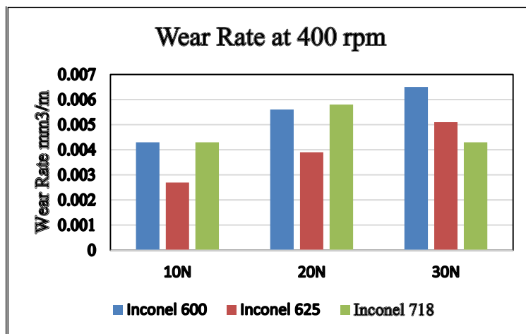
Figure 5 Wear rate at 400 rpm
