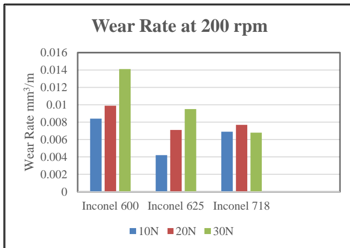
Figure 3. Wear rate at 200 rpm
