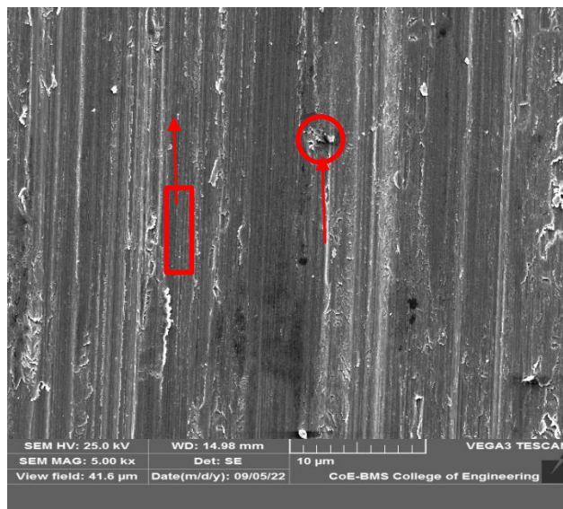
Figure 7 worn-out surfaces for the Inconel 600- Cr_3C_2 -NiCr coatings for the speed of 300 rpm and load of 20N
