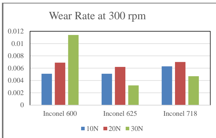
Figure 4 Wear rate at 300 rpm
