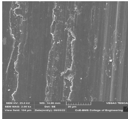
Figure 13 worn-out surfaces for the Inconel 718- \text{Cr}_3\text{C}_2 -NiCr coatings for the speed of 300 rpm and load of 20N
