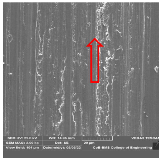
Figure 10 worn-out surfaces for the Inconel 625- Cr 3 C 2 -NiCr coatings for the speed of 300 rpm and load of 20N
